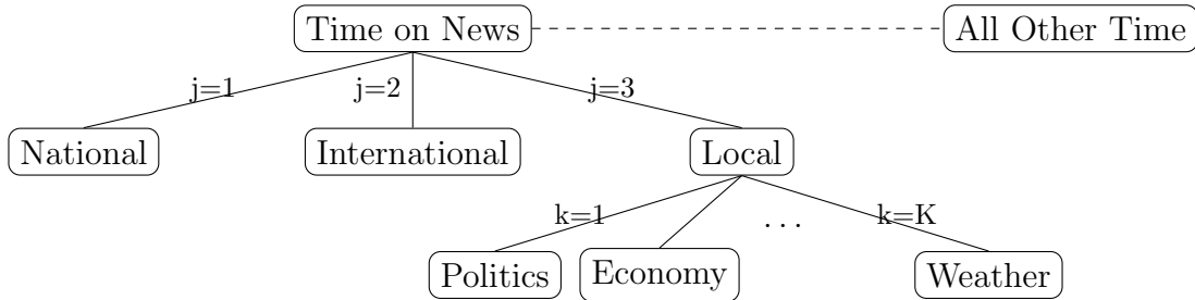
Figure 1: Information Structure
